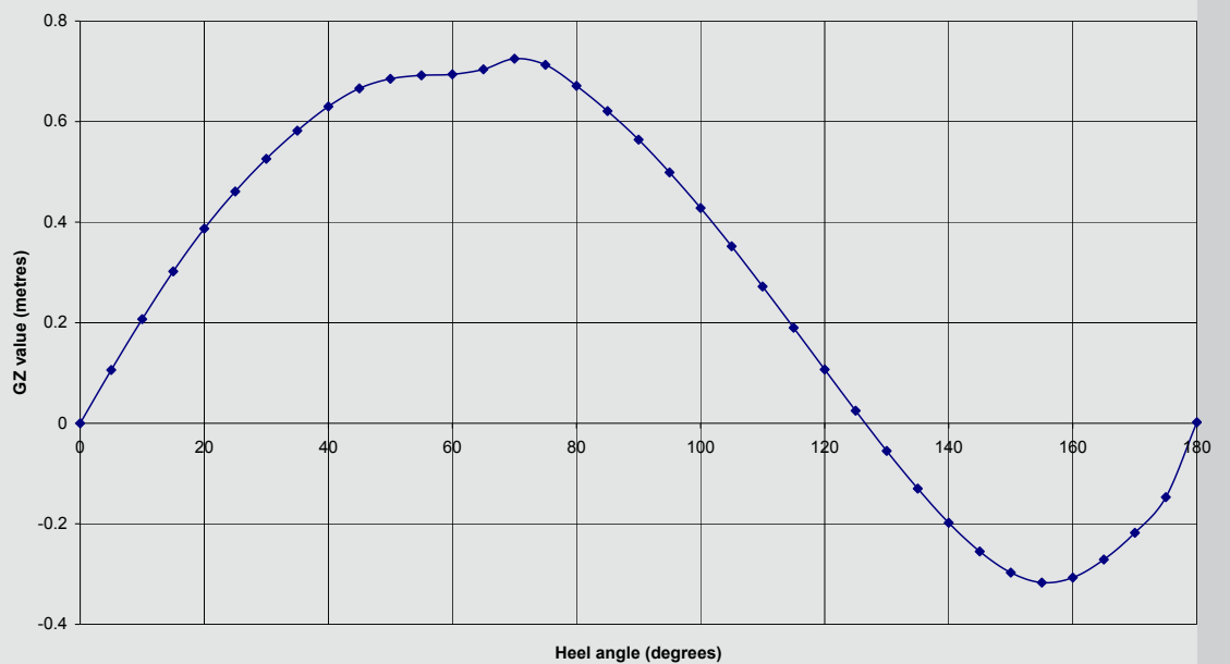
Stability curve
